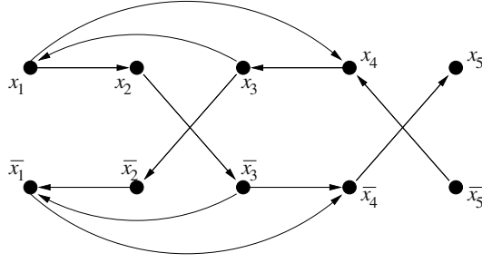
Figure 7.2: Digraph G(F_1) .
